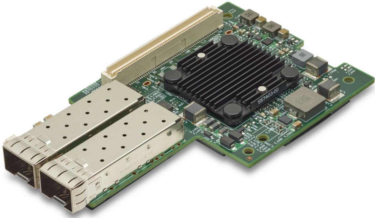
Figure 1: BCM957414M4142C OCP 2.0 Mezzanine Card
